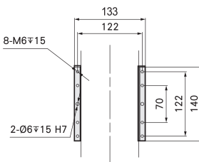
B-Detail View
