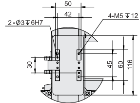
B-Detail View
